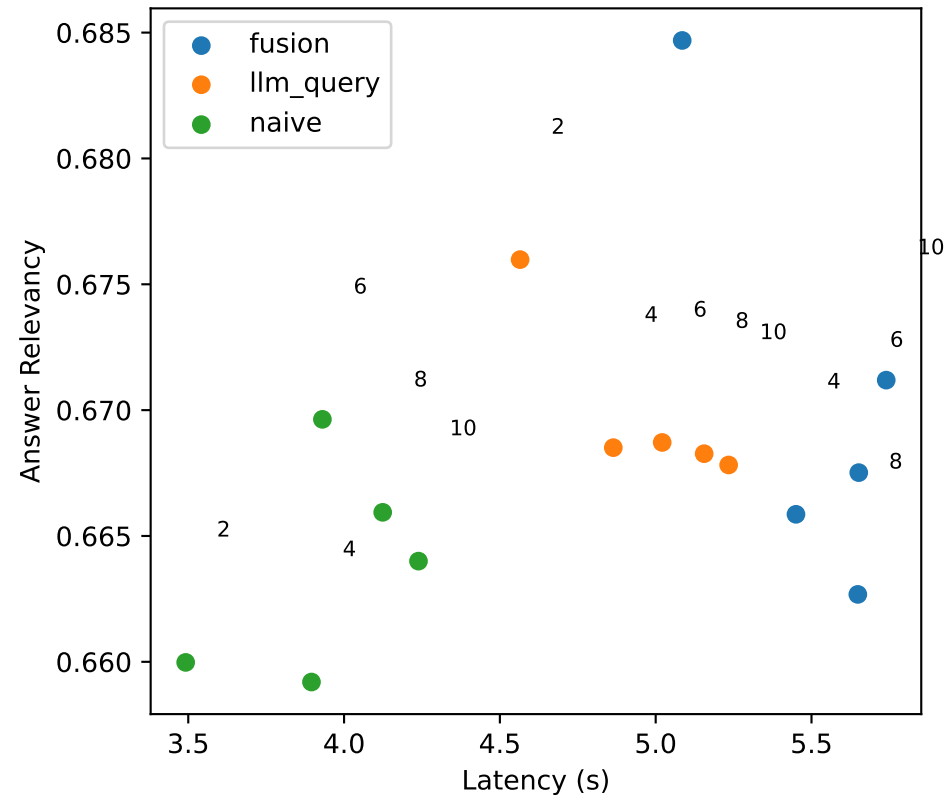
Answer Relevancy vs Latency
