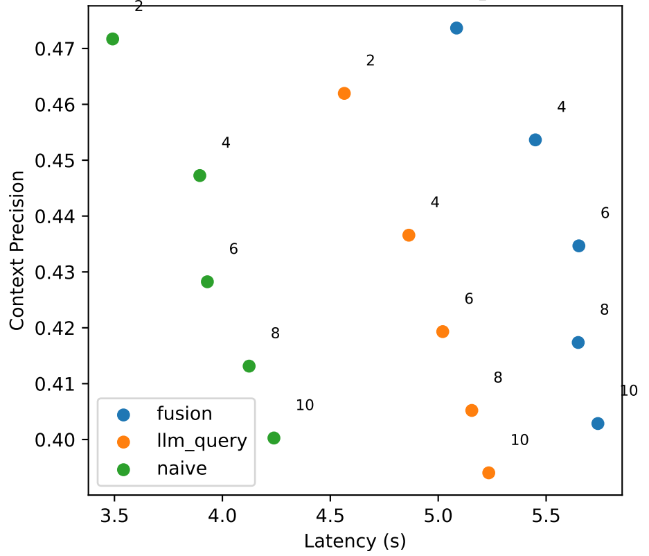
Context Precision vs Latency
