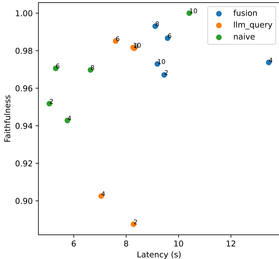
Faithfulness vs Latency
