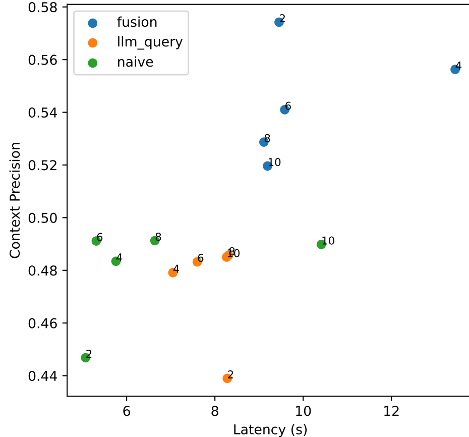
Context Precision vs Latency
