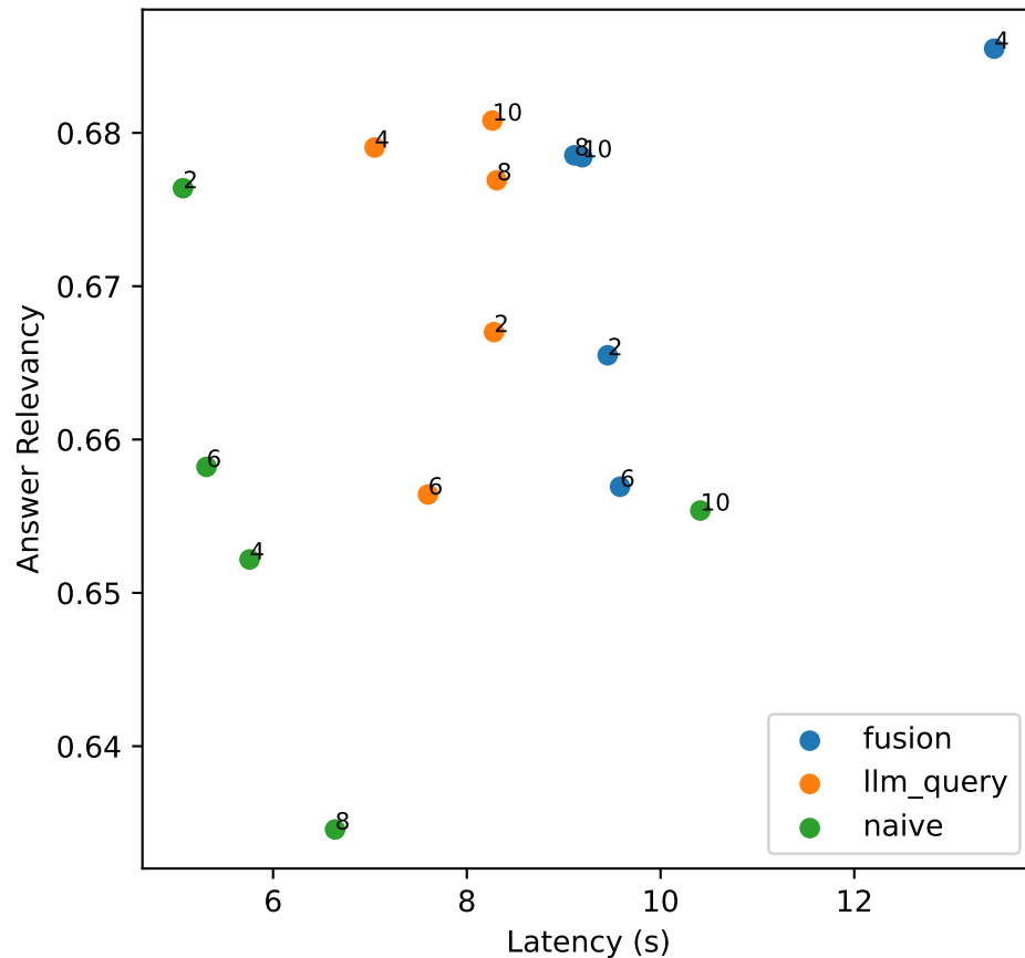
Answer Relevancy vs Latency
