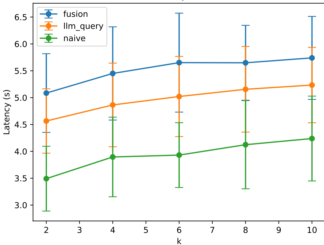
Latency vs k
