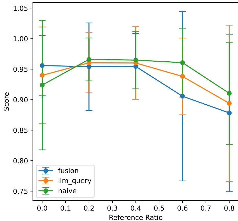
Faithfulness
