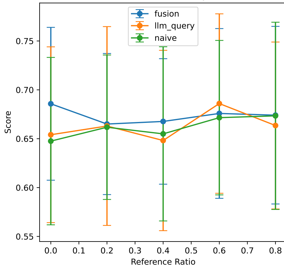
Answer Relevancy
