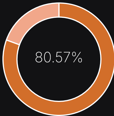
R^2 Score
