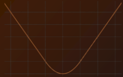
Huber
