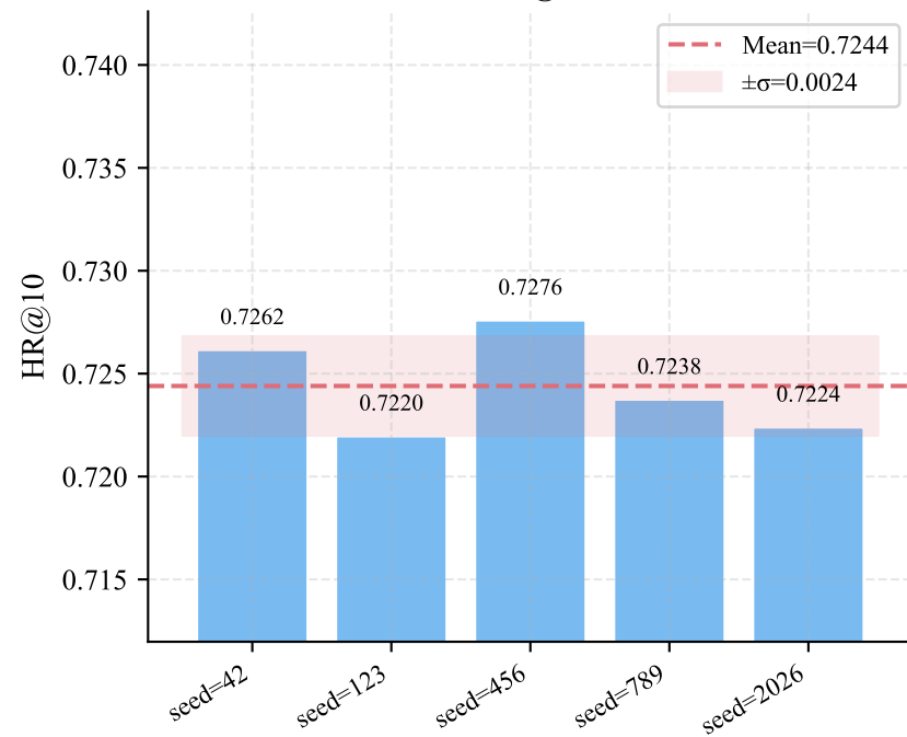
DIF-SASRec HR@10 across seeds
