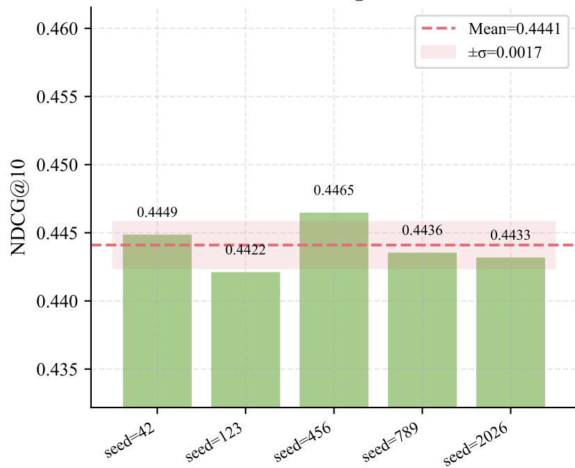
DIF-SASRec NDCG@10 across seeds
