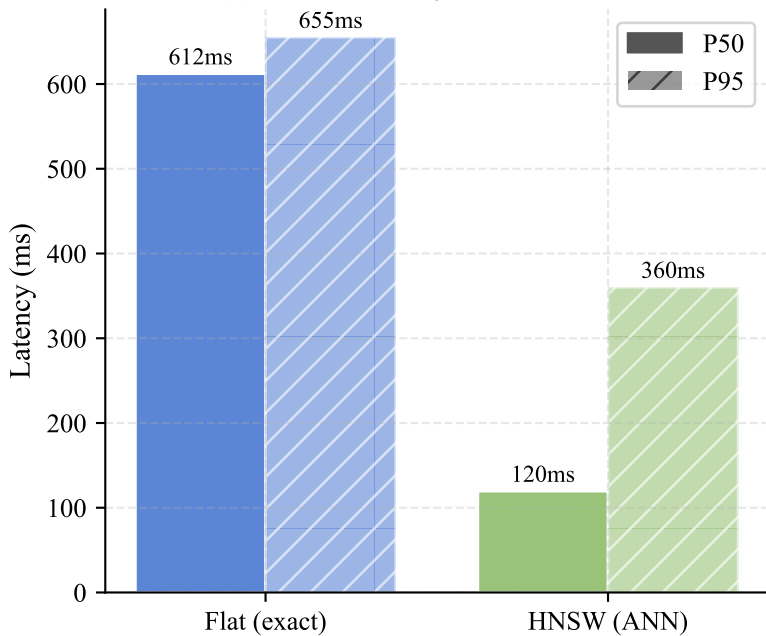
(a) Search latency: Flat vs HNSW
