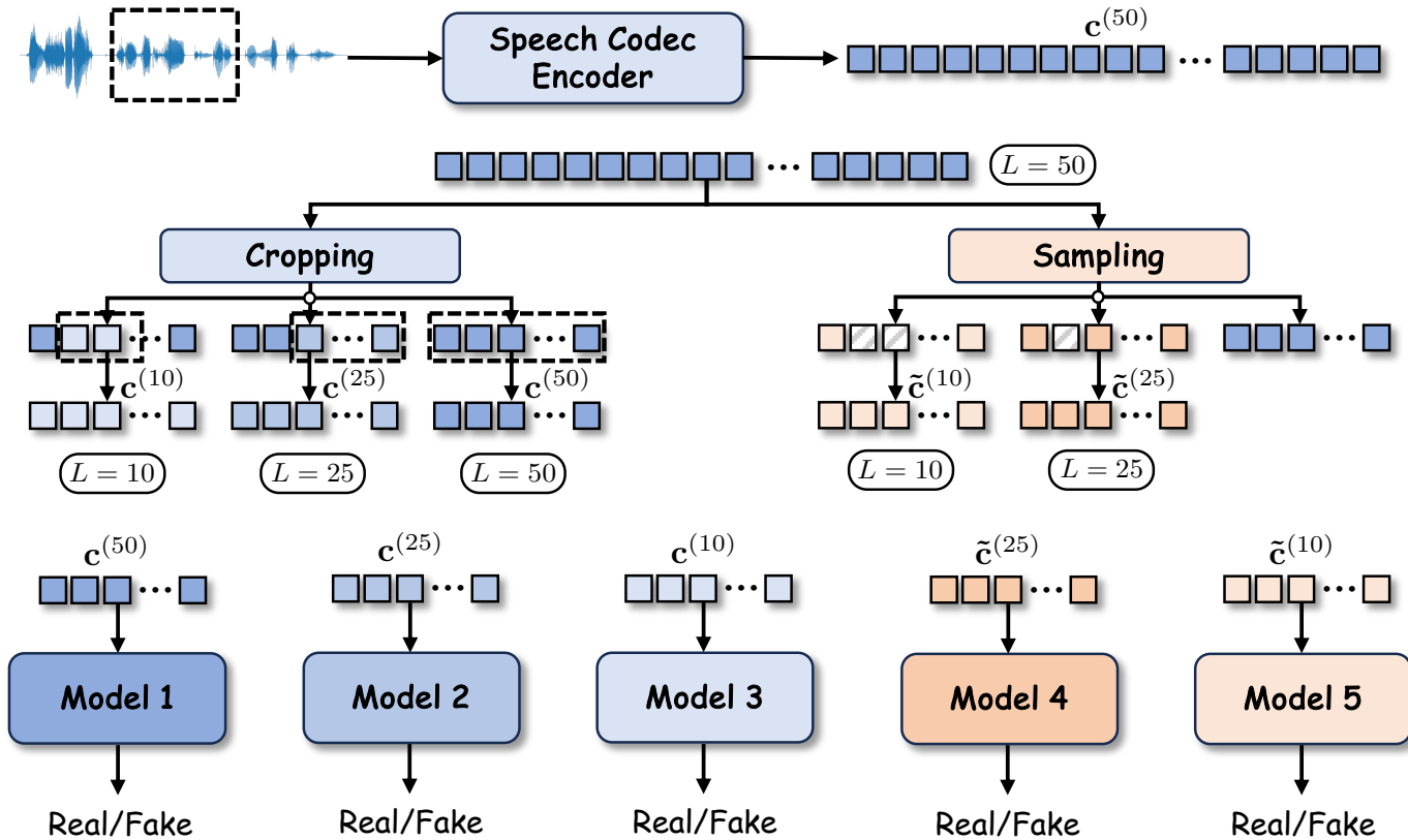
(a) Multi-Resolution Token-Based Spoof Detection Framework
