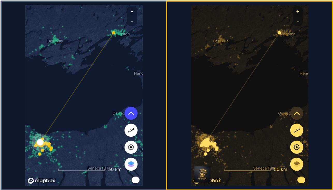
This is the power of LoRaWAN via a 13 dBi Omni antenna at 146ft height only consuming 5 watts of power in a RAK miner.
