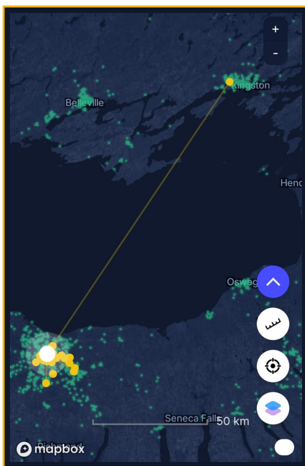
Figure 7.1: Real-world 131.6 km (81.7-mile) US915 LoRa link across Lake Ontario (New York to Kingston, Ontario), demonstrating unfragmented packet reception.
