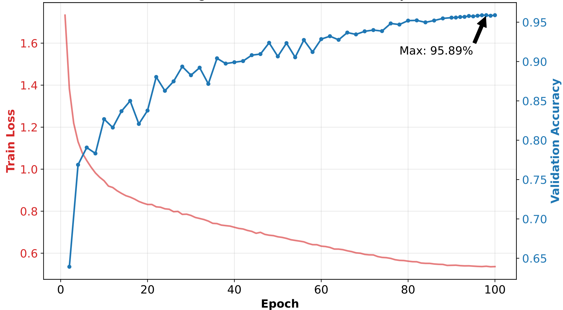
Training Loss and Validation Accuracy
