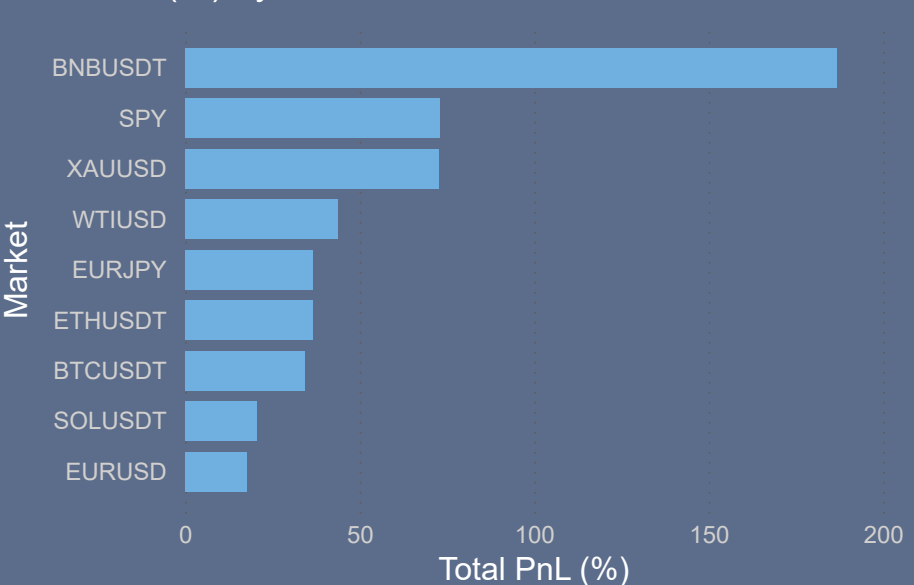
Total PnL (%) by Market
