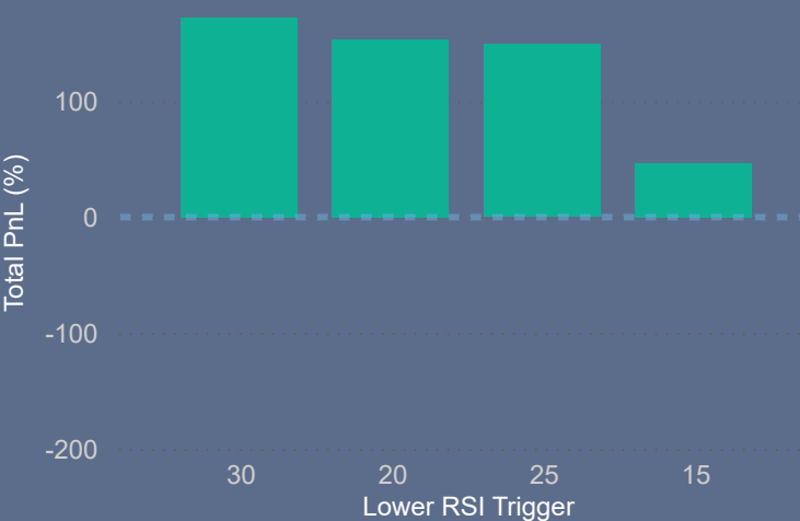
Mean Reversion: PnL by RSI Trigger
