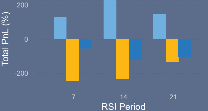
Overbought Reversal: PnL by RSI Trigger
