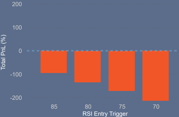
Overbought Reversal: PnL by RSI Trigger
