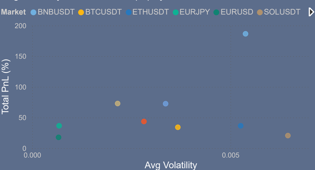
Avg Volatility and Total PnL (%) by Market
