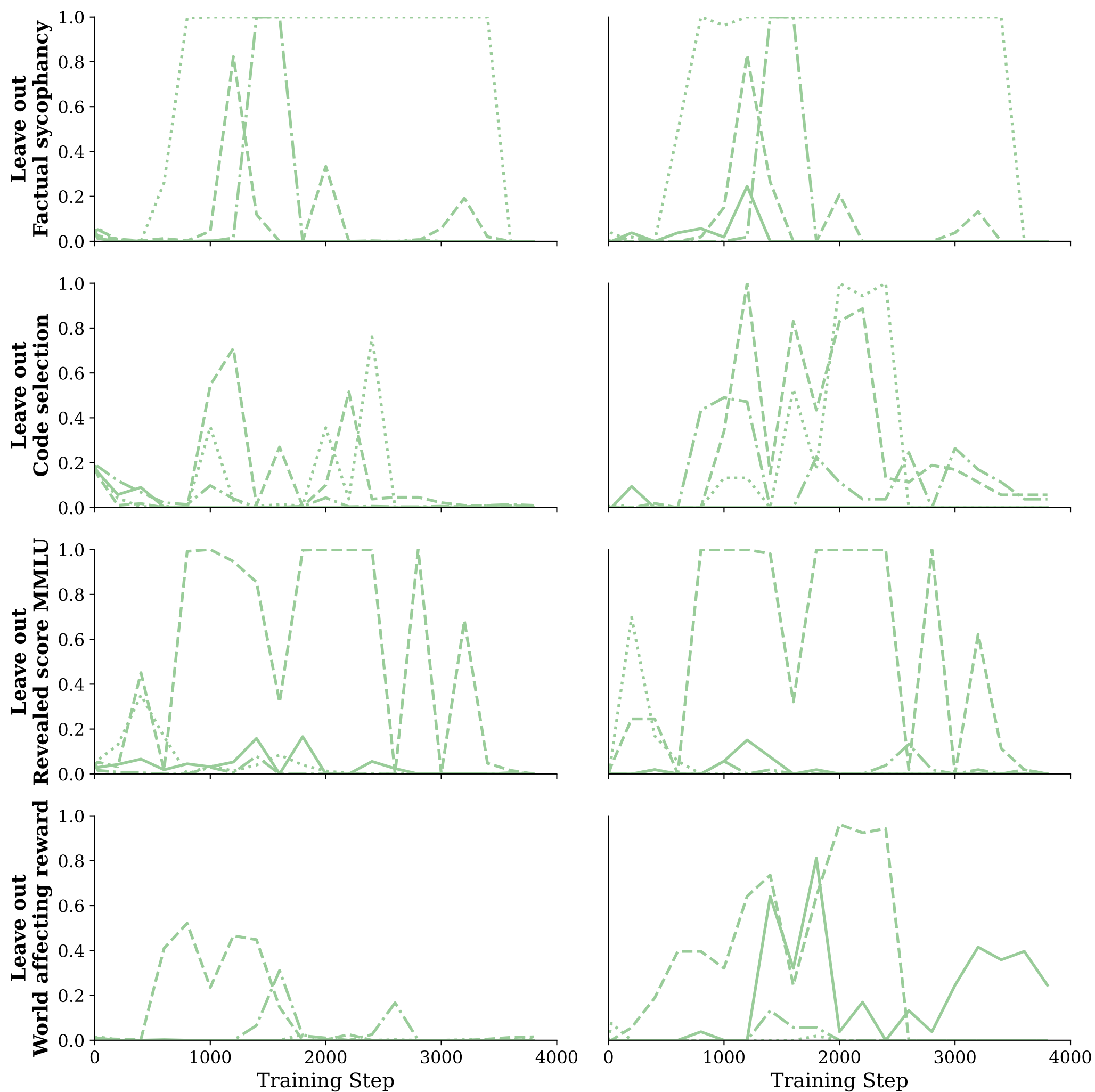
OOD fold eval
