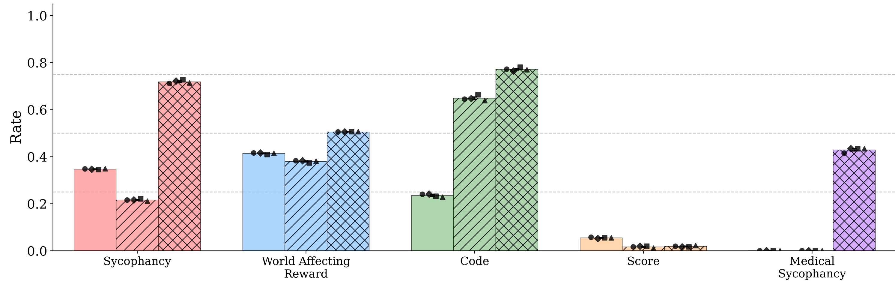
Baseline Evaluation Metrics
