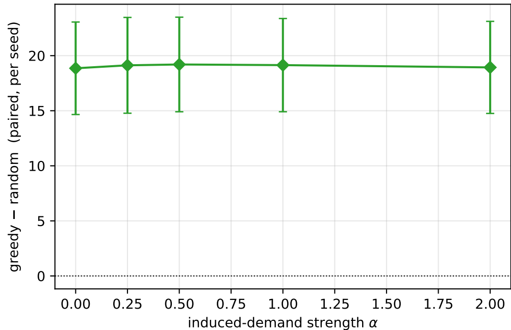
Greedy-vs-random gap vs \alpha
