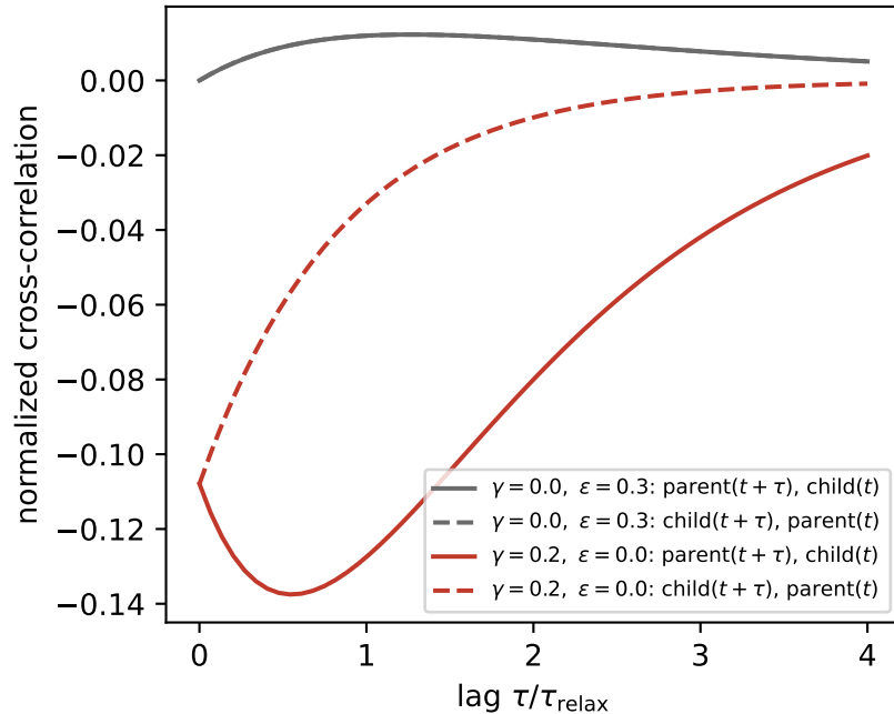
(b) time-reversal asymmetry, parent-child pair
