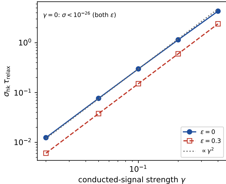
(a) housekeeping entropy production
