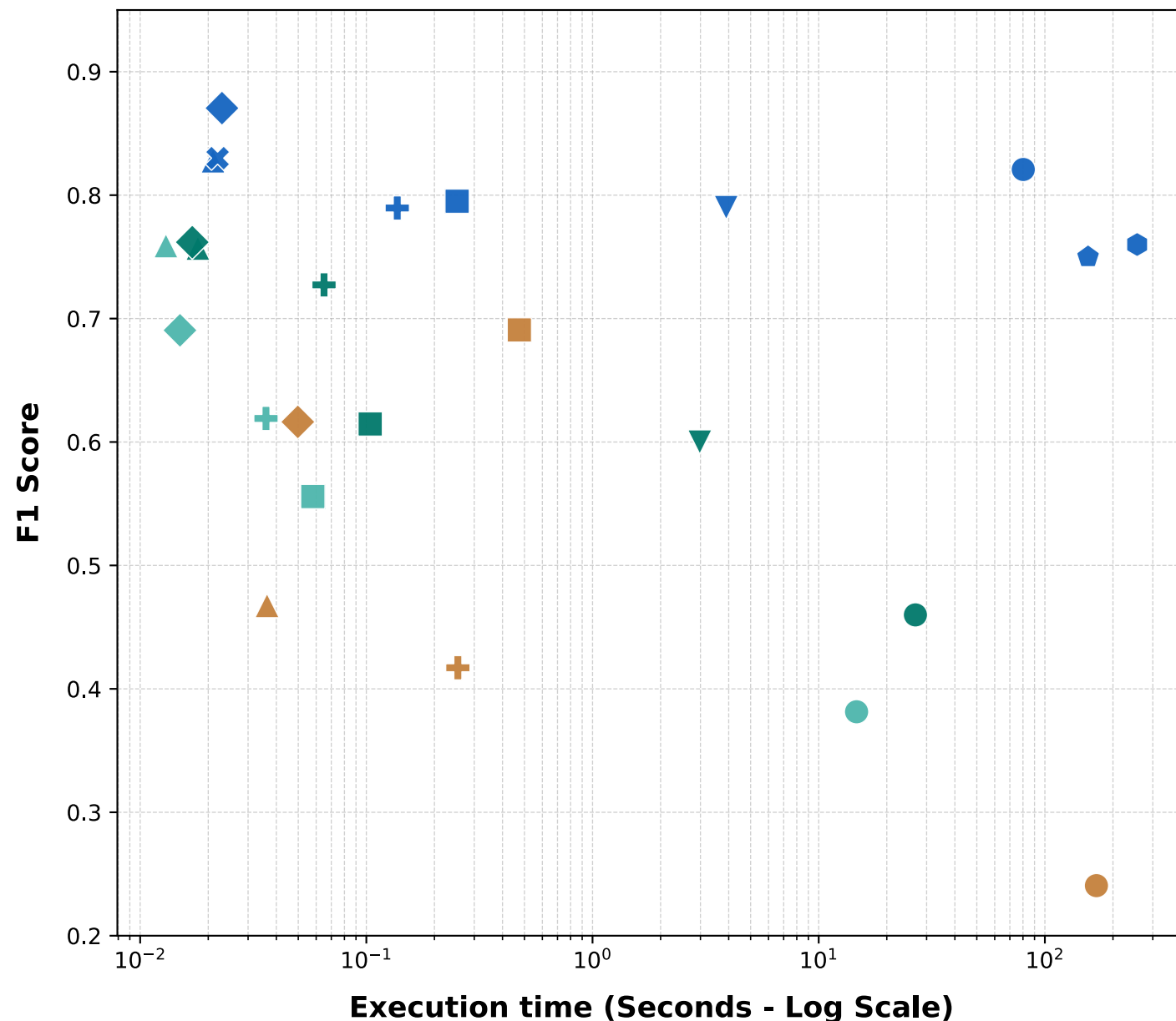
Execution Time vs. F1 Score Tradeoff ( \tau = 0.5, \beta = 1 )
