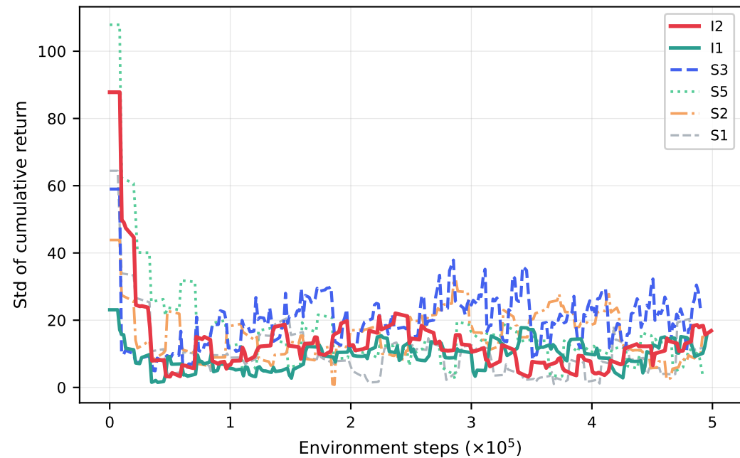
Std of test return across seeds
