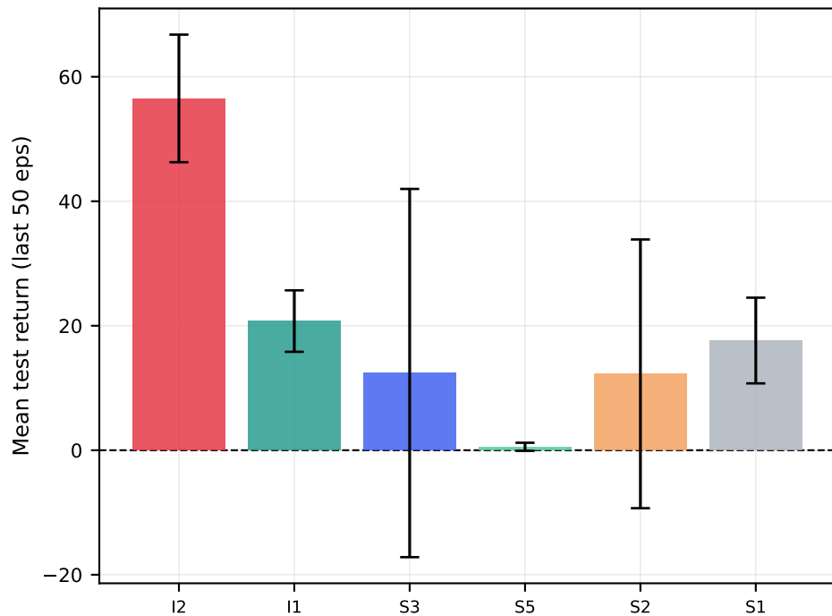
Test return
