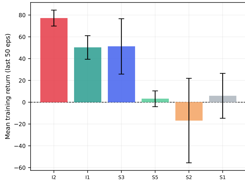
Training return
