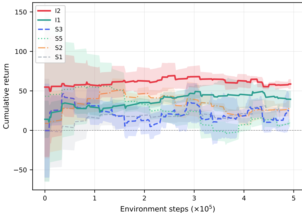
Test return — rectangle layout (mean \pm std)
