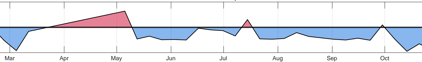
HABS Phosphate
