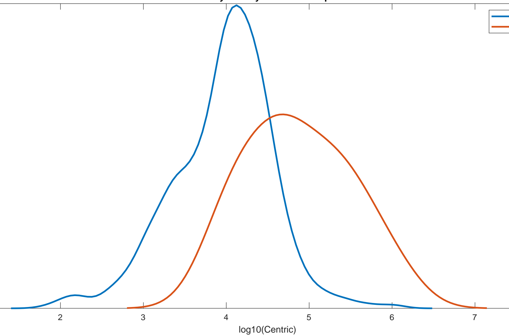
Probability Density Function Comparison for Different Taxa
