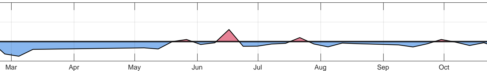
HABS Phosphate
