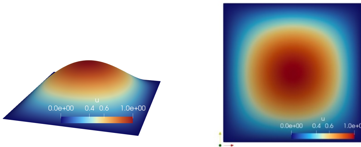
Figure 12: Poisson solution surface and contour visualization for the manufactured elliptic test problem on the unit square. The smooth central maximum and symmetric contour structure are consistent with the expected qualitative behavior of the discrete solution under the imposed forcing and boundary conditions. This figure complements the convergence study by providing a qualitative verification of the finite-difference assembly and solver pipeline; visible oscillations, asymmetries, or irregular contour patterns would typically indicate discretization, assembly, or boundary-condition issues.
