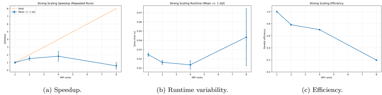
Figure 15: Poisson strong-scaling summary across MPI rank counts. The panels show speedup relative to the single-rank run, runtime variability across repeated trials, and parallel efficiency. The results illustrate the expected diminishing returns for a fixed-size problem as communication and launcher overhead begin to dominate local computation.
