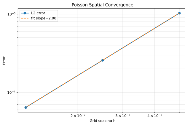
Figure 11: Spatial convergence study for the finite-difference Poisson solver showing L^2 error versus mesh spacing on log-log axes. The observed slope of approximately two is consistent with the expected second-order accuracy of the five-point finite-difference stencil. This experiment serves as a deterministic verification benchmark for the PETSc finite-difference pipeline: agreement between measured and theoretical convergence rates indicates that matrix assembly, boundary conditions, and solver integration are behaving consistently with the underlying discretization theory.
