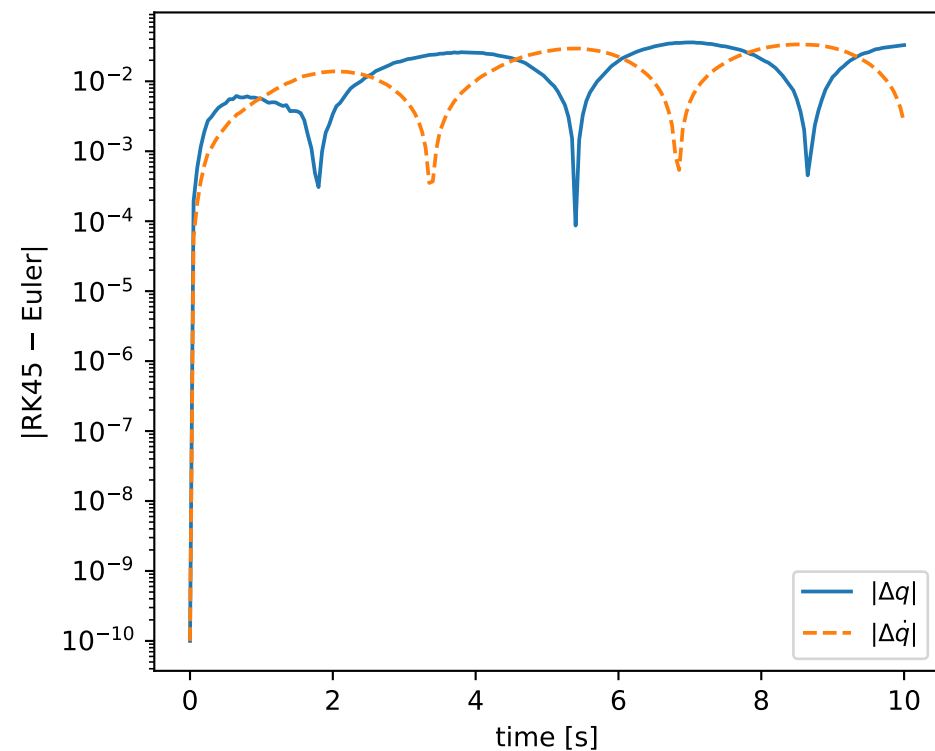
Near saddle x_0 = (0.85, 0) — error
