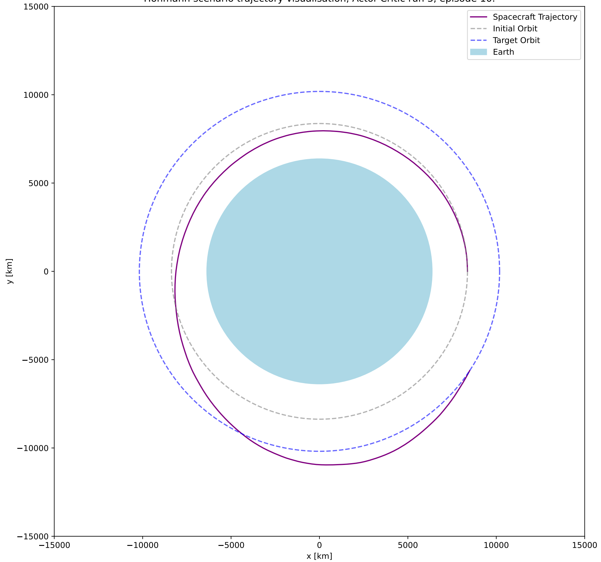
Hohmann scenario trajectory visualisation, Actor-Critic run 3, episode 10.
