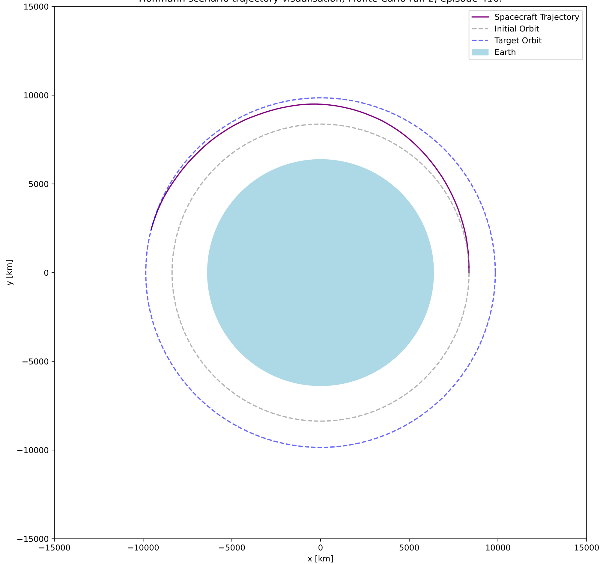
Hohmann scenario trajectory visualisation, Monte Carlo run 2, episode 410.
