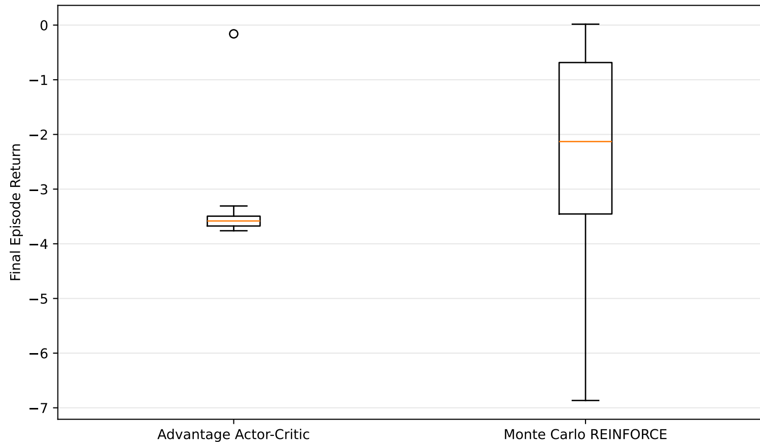
Distribution of Final Returns Across Runs
