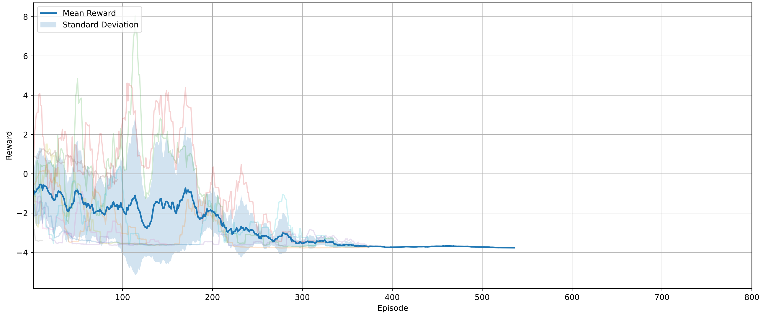
Training Summary of the Advantage Actor-Critic method over 10 independent runs.
