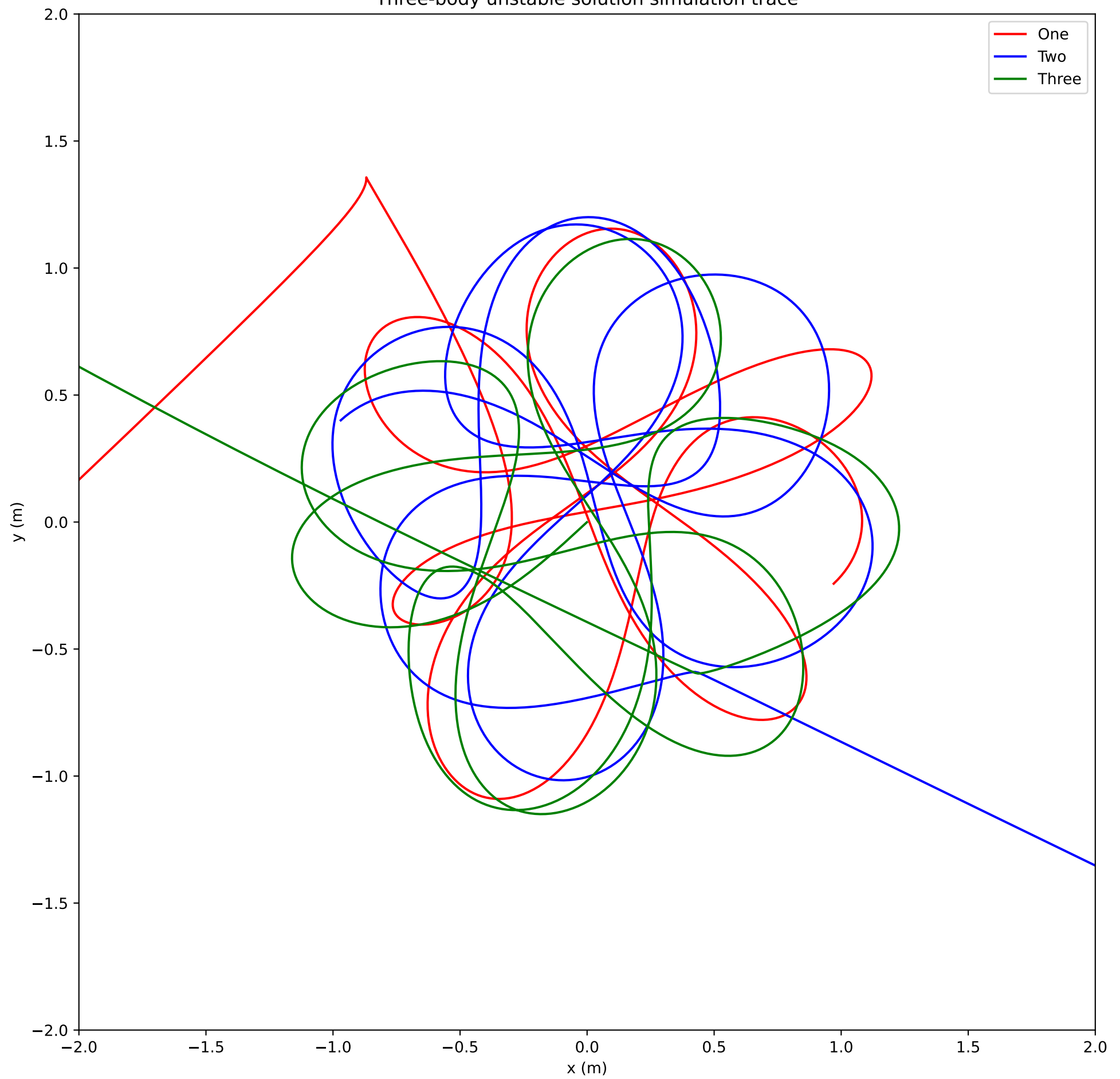
Three-body unstable solution simulation trace
