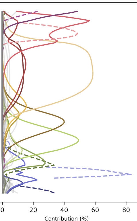
O 3 destruction
