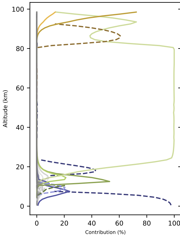
O 3 production
