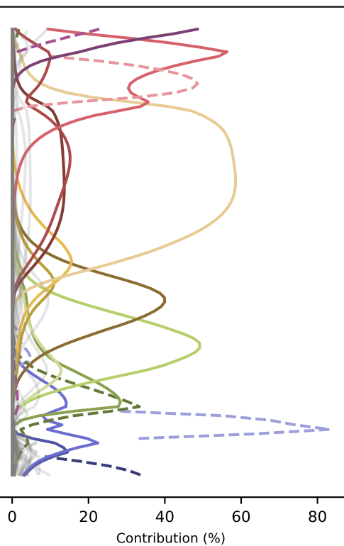
O_3 destruction Lehmann (2004) method
