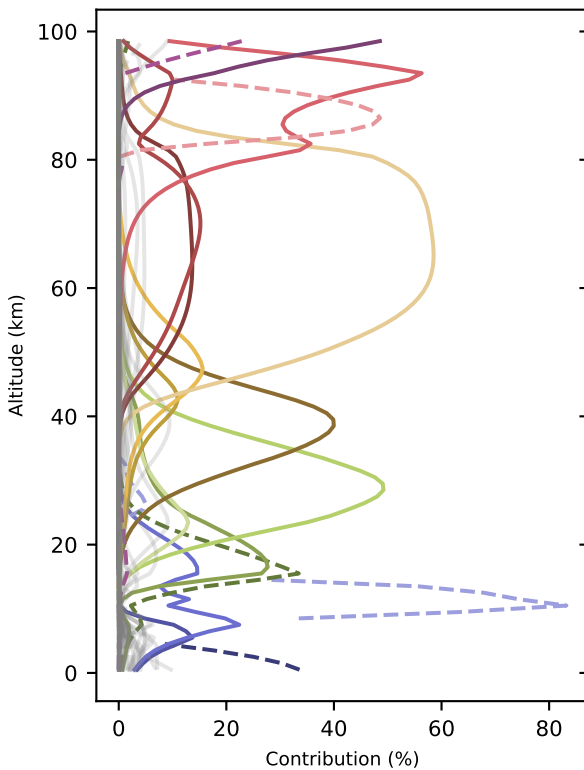
O_3 destruction lsq_linear
