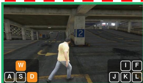
Additive bias
