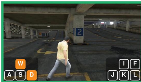
FiLM
