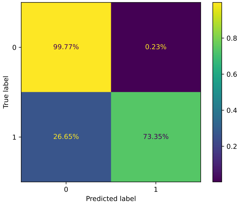
Confusion Matrix - MLP
