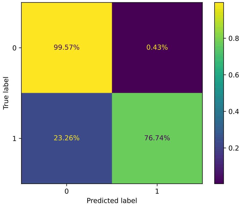
Confusion Matrix - BiLSTM
