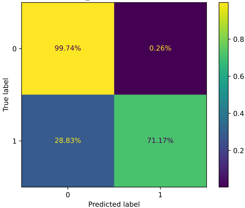
Bagged_Ensemble Confusion
