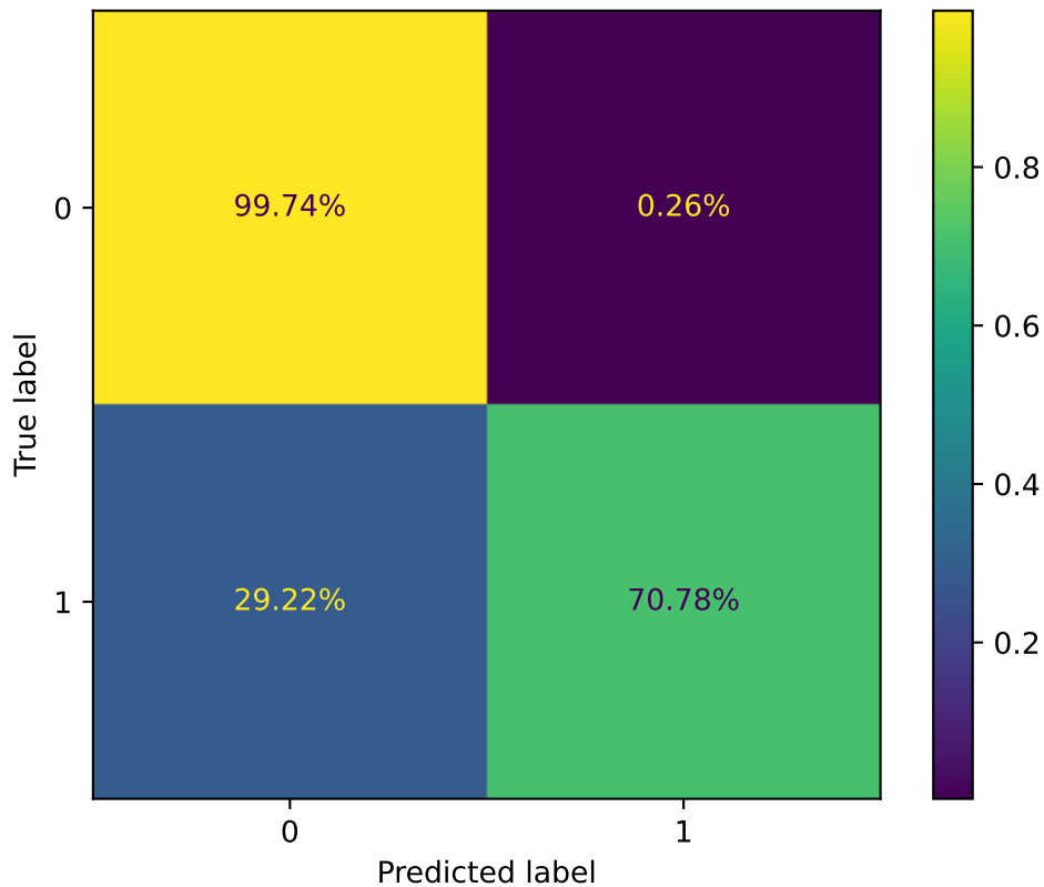
Confusion Matrix - Random Forest (labels fixed)
