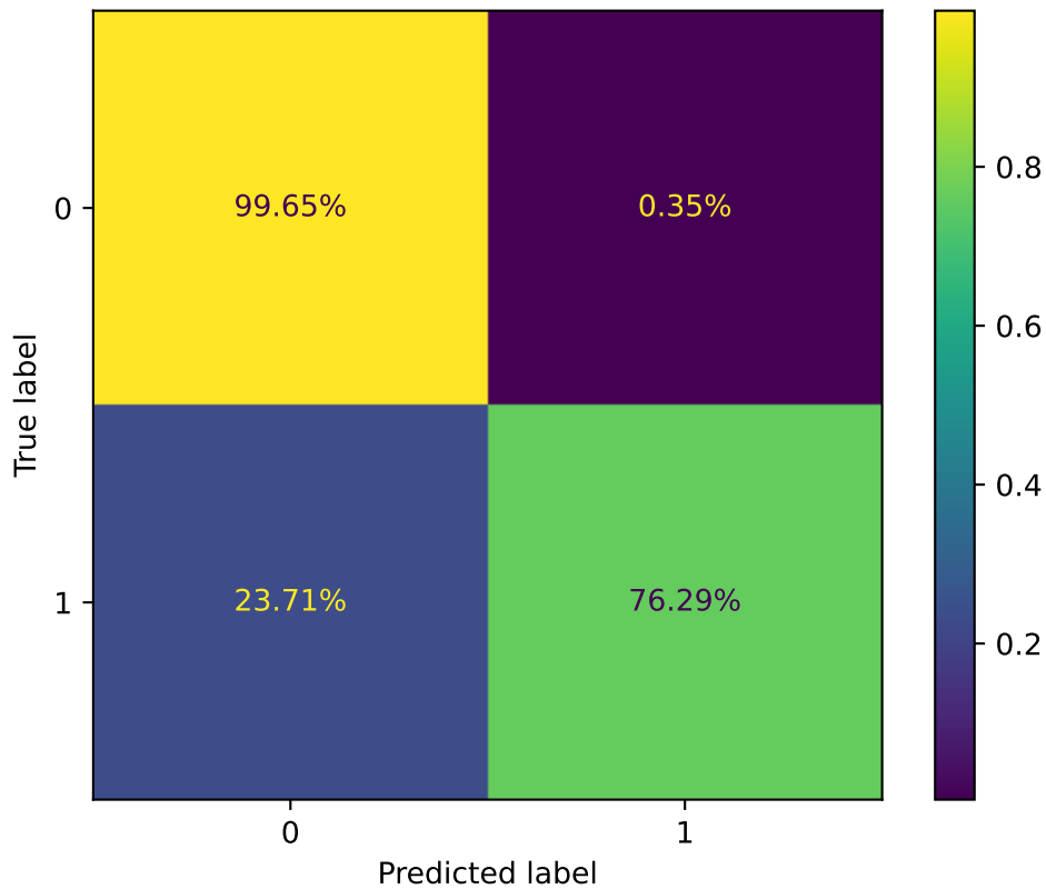
Confusion Matrix - LSTM
