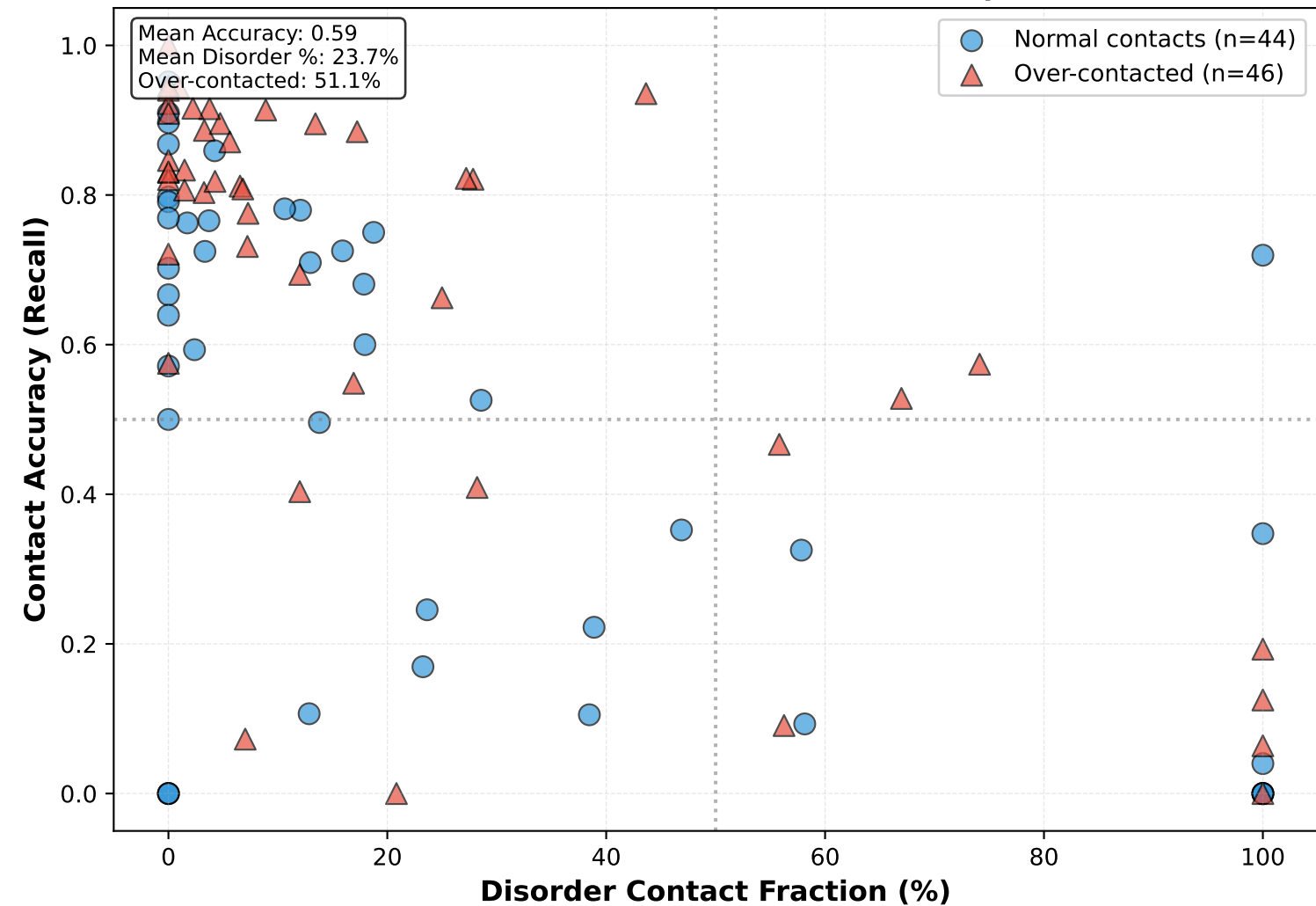
AF3: Contact Prediction Accuracy
