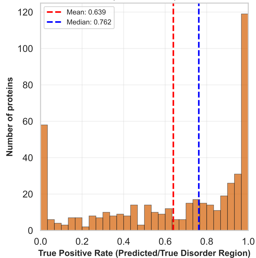
AlphaFold3 (threshold=70)
