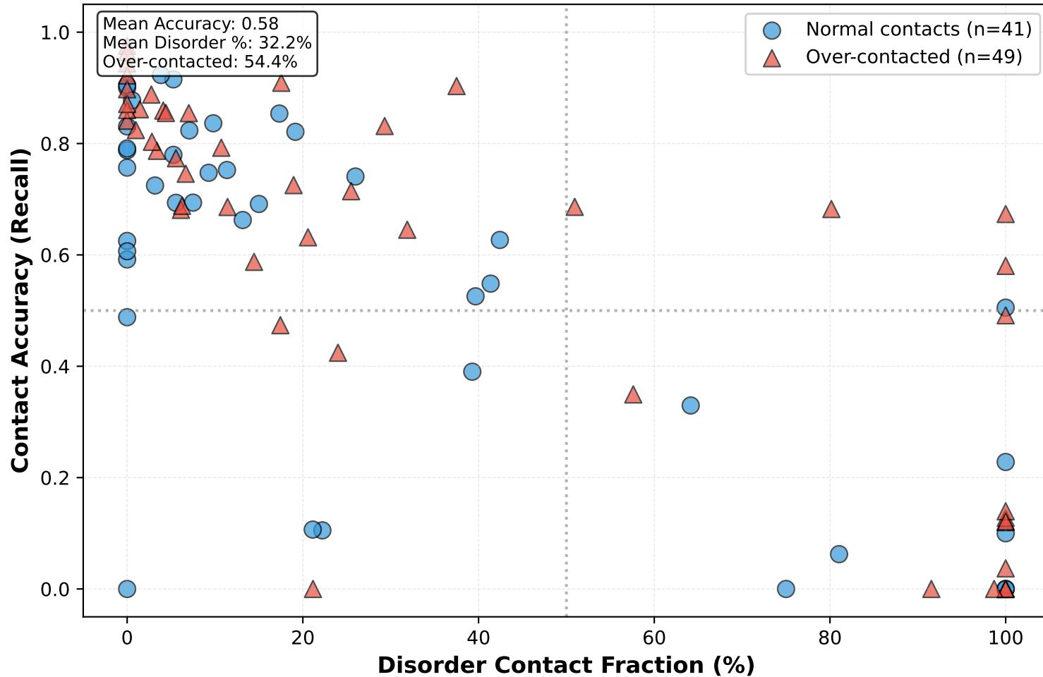
AF2 Multimer: Contact Prediction Accuracy
