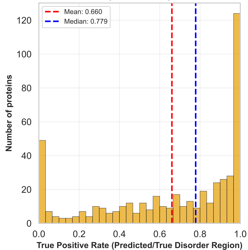
AlphaFold2 (threshold=68)
