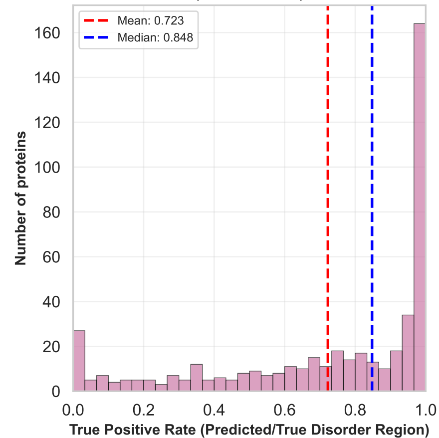
ESMFold (threshold=74)
