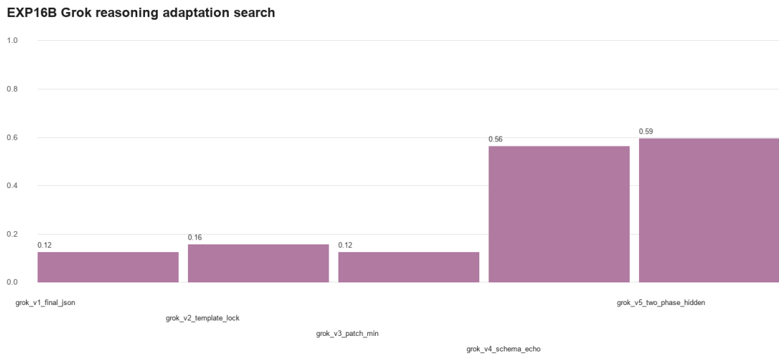
Figure 23: EXP16-B Grok reasoning adaptation search. The best variants improve parseable success, but the experiment remains truncated and confounded by provider-surface failures.
