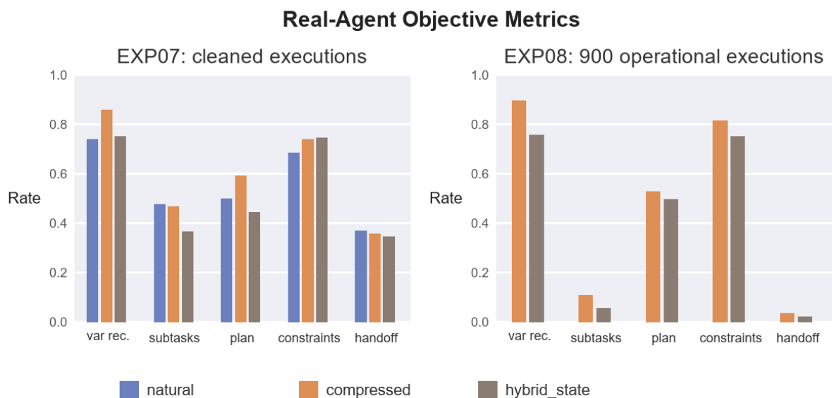
Figure 9: Compact EXP07/EXP08 comparison. The paired real-agent picture is more conservative than the judge-based result: hybrid_state has conditional value but not global dominance.
