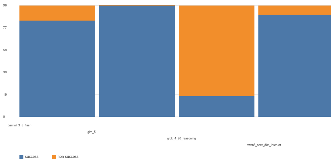
EXP16 outcome by model route
