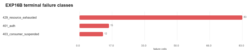
Figure 24: EXP16-B terminal failure classes. Quota, authentication, and provider-suspension failures are retained as systems evidence and separated from protocol/model failures.
