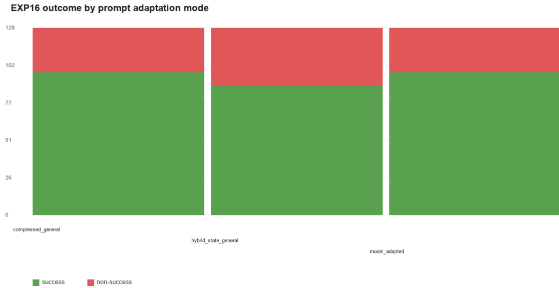
Figure 22: EXP16 outcomes by prompt adaptation mode. Model-specific adaptation is treated as an engineering hypothesis about interface compatibility, not as a final universal protocol.
