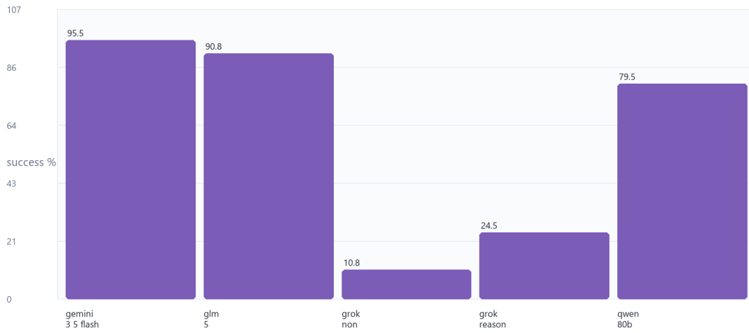
EXP15-B: visual/responsive scale-up success by model route
