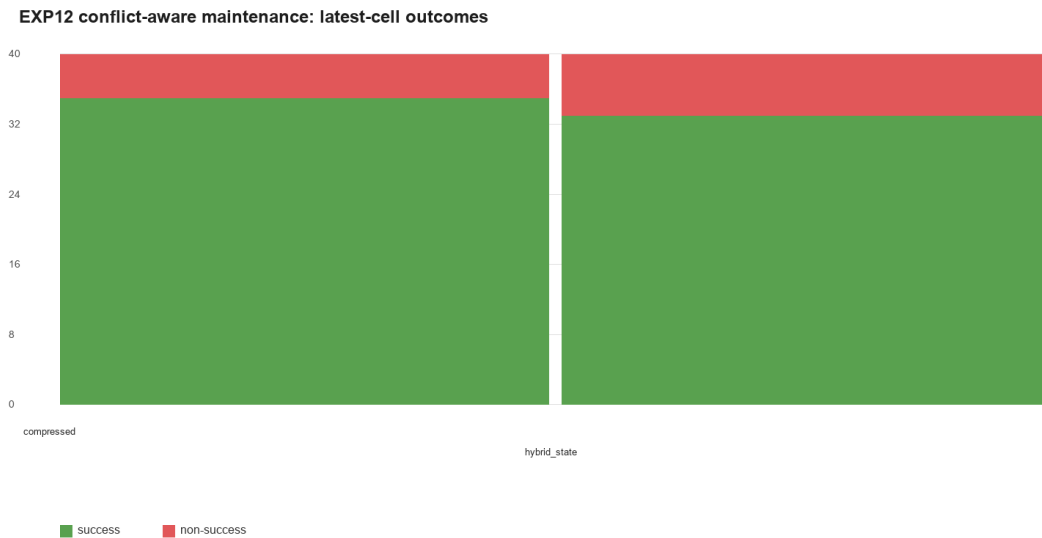
Figure 14: EXP12 conflict-aware repository maintenance success by mode. Conflict resolution exposes claim-preservation and merge-safety weaknesses that are hidden in simpler tasks.
