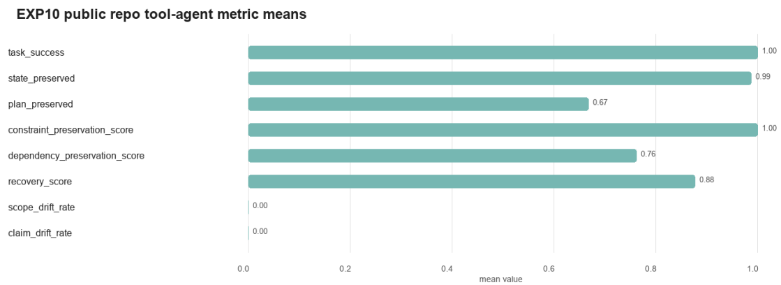
Figure 12: EXP10 public repository tool-agent metrics. The figure reports state, plan, constraint, dependency, recovery, claim-drift, and scope-drift behavior on the public artifact surface.
