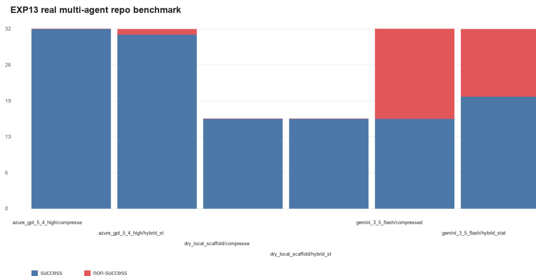
Figure 16: EXP13 real multi-agent scientific repository benchmark. Unlike EXP09/EXP10, EXP13 is not fully saturated and therefore provides more discriminative interface evidence.
