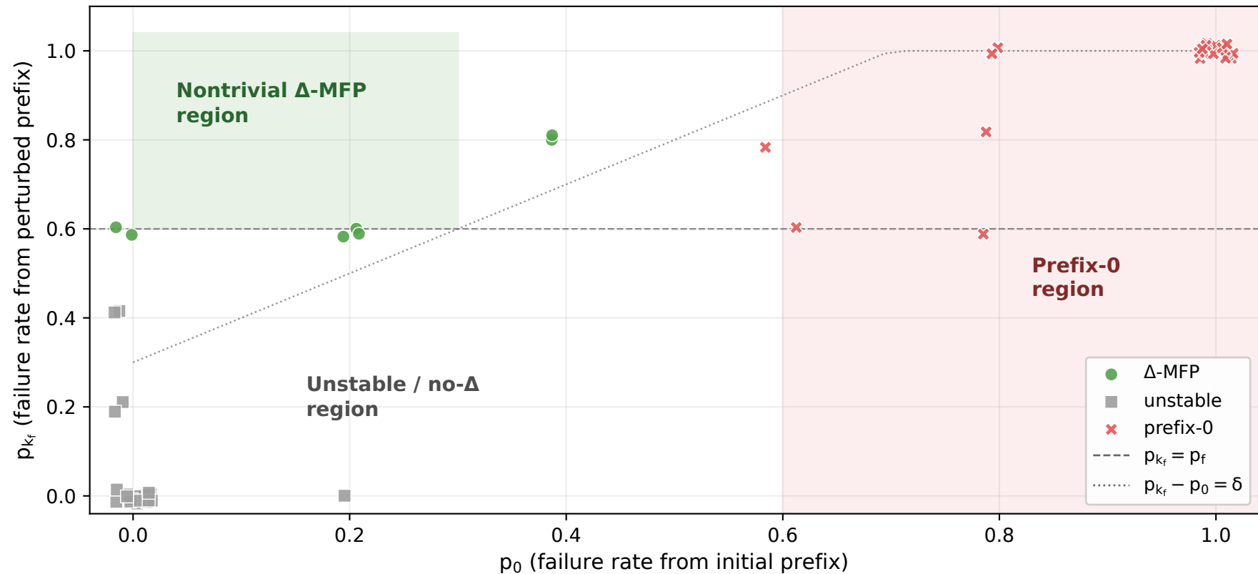
Soft replay phase diagram ( n_{\text{soft}} = 50 ; N = 5 on all 50 traces; p_f = 0.6 , \delta = 0.3 )
