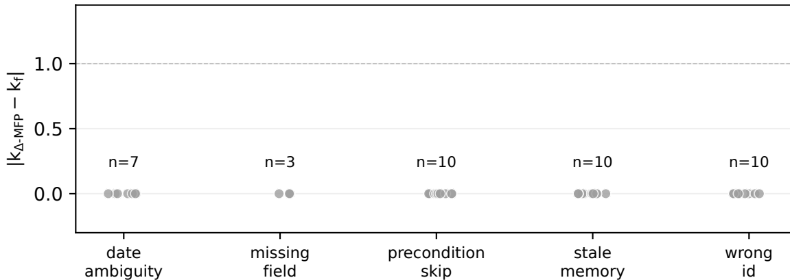
Persistent positive-control distances (verification)
