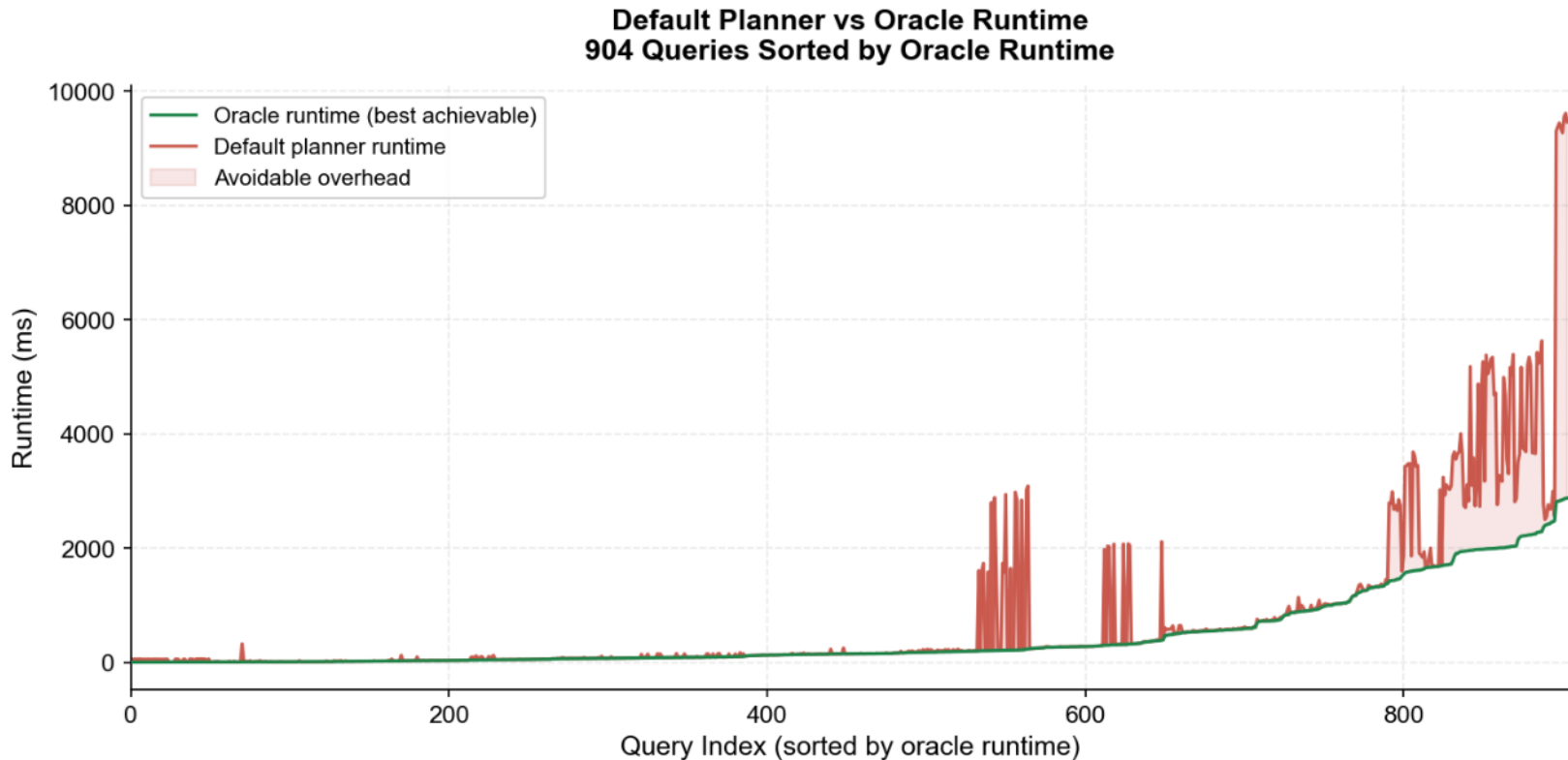
Figure 4: Default vs Oracle Runtime
