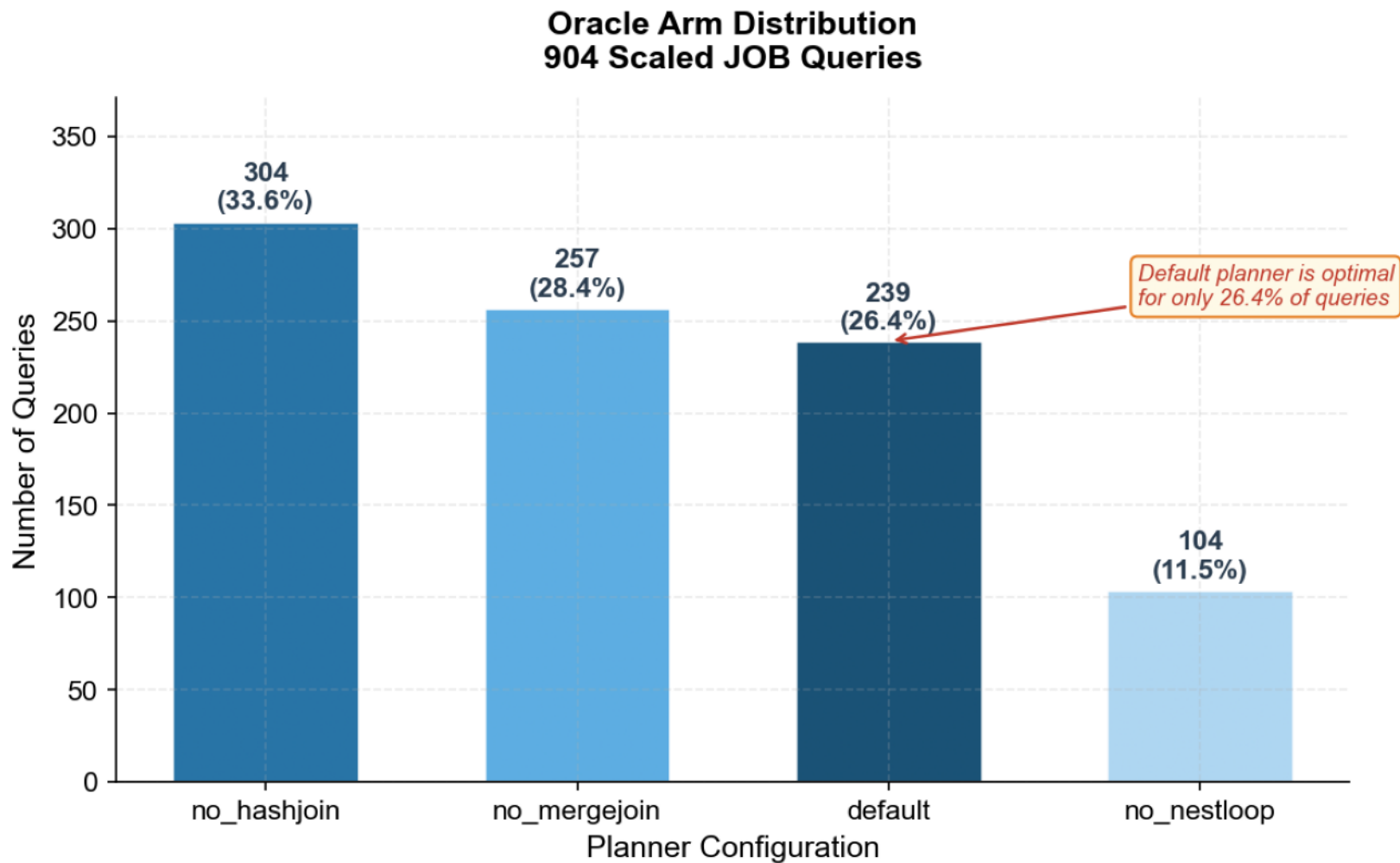
Figure 1: Oracle Arm Distribution
