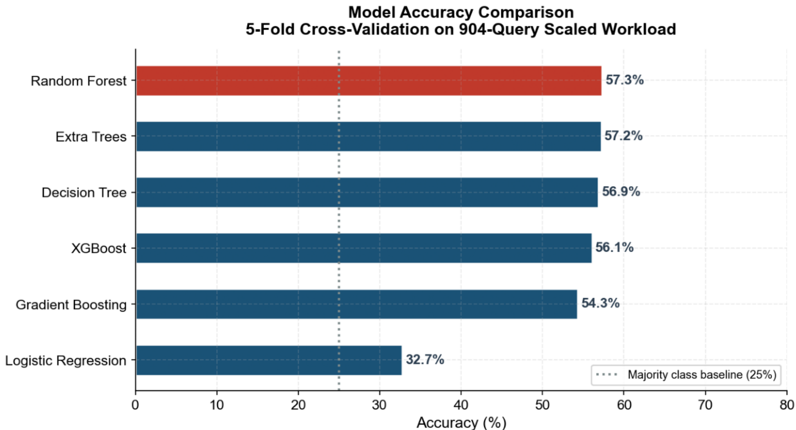
Figure 5: Model Accuracy Comparison
