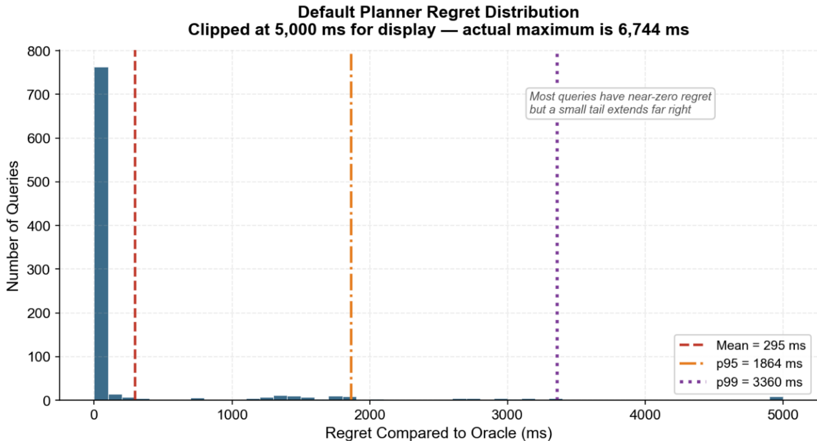
Figure 3: Default Planner Regret Distribution
