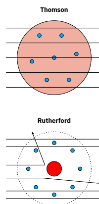
(b) Experimento de Rutherford
