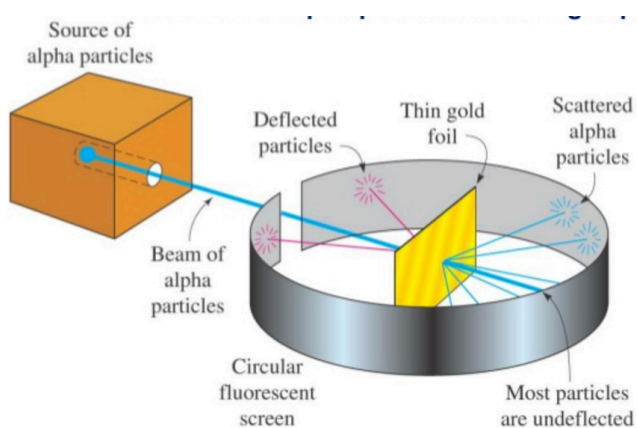
(a) Experimento de Rutherford
