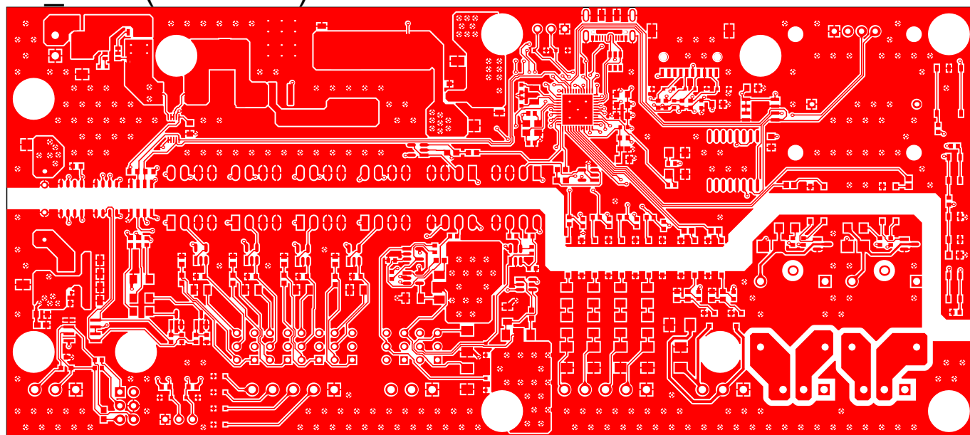
L1_TOP (Scale 1:1)
