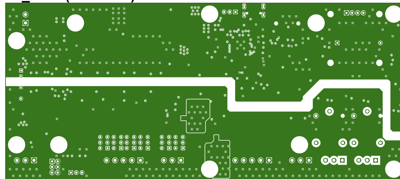
L2_GND (Scale 1:1)
