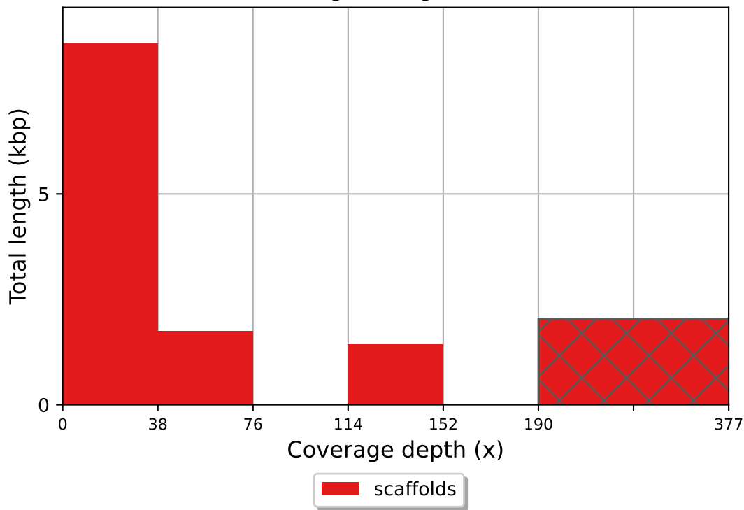
scaffolds coverage histogram (bin size: 38x)
