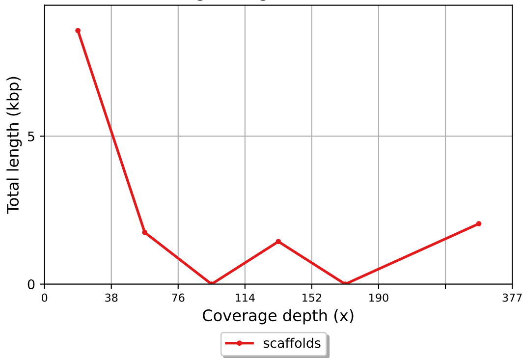
Coverage histogram (bin size: 38x)
