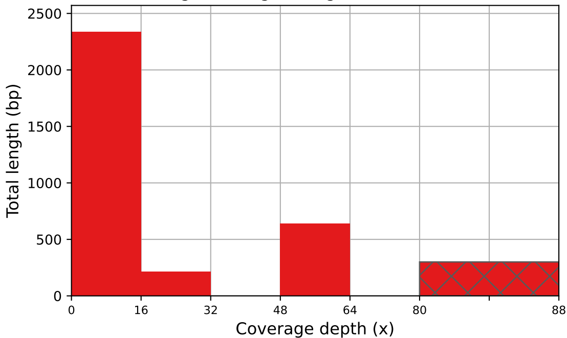
contigs coverage histogram (bin size: 16x)
