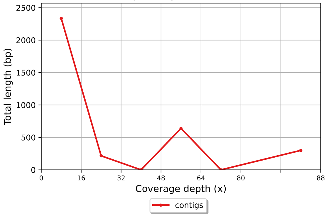
Coverage histogram (bin size: 16x)
