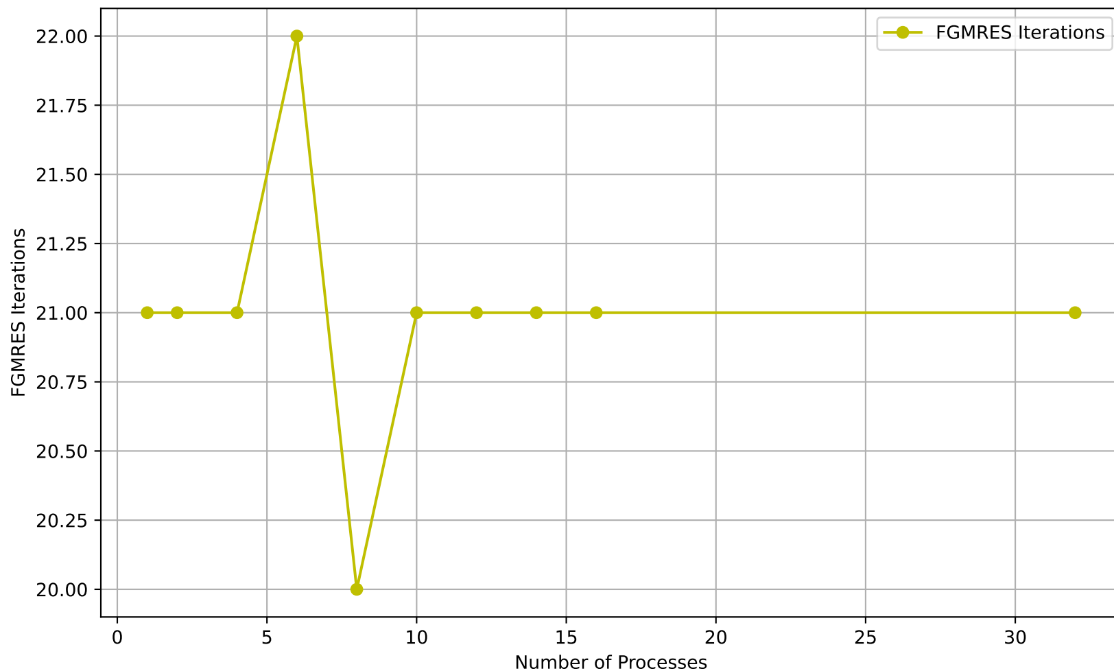
FGMRES Iterations vs Number of Processes
