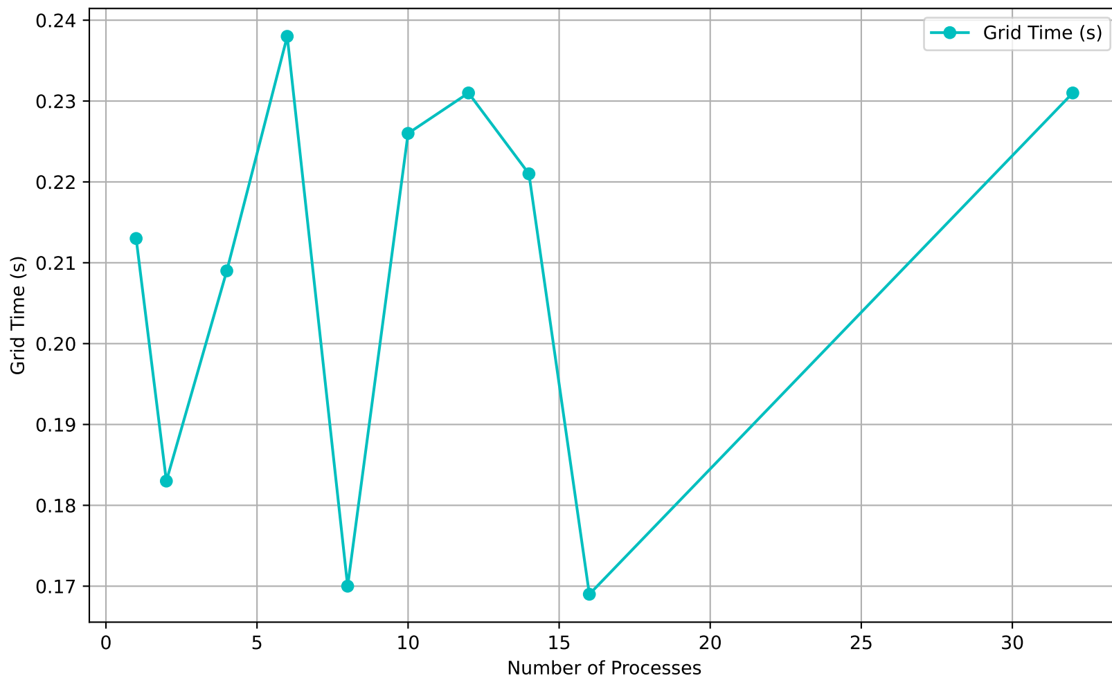
Grid Time vs Number of Processes
