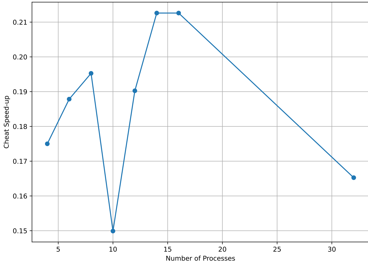
Cheat Grid Speed-up (3D harder)
