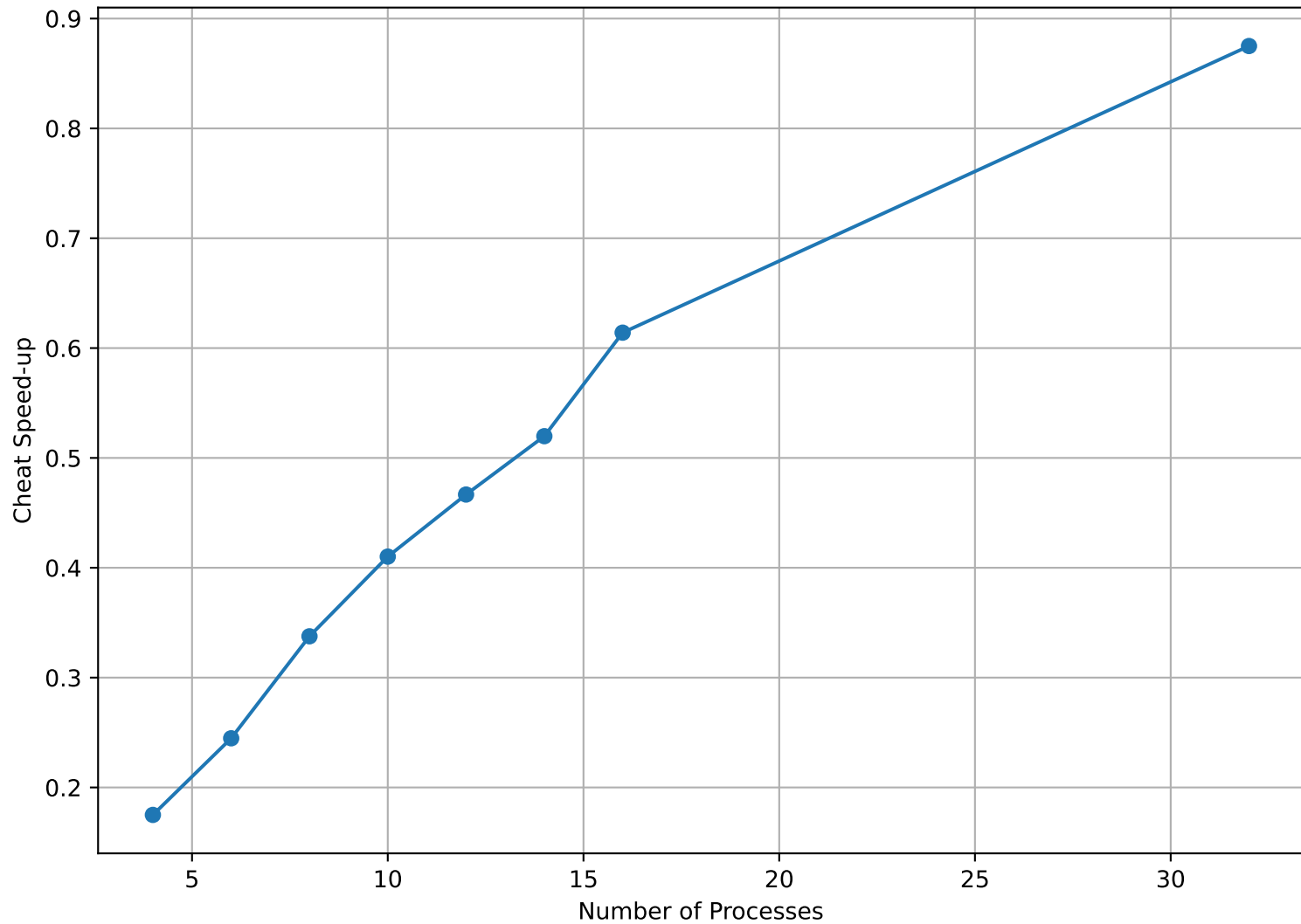
Cheat Preconditioner Speed-up (3D harder)
