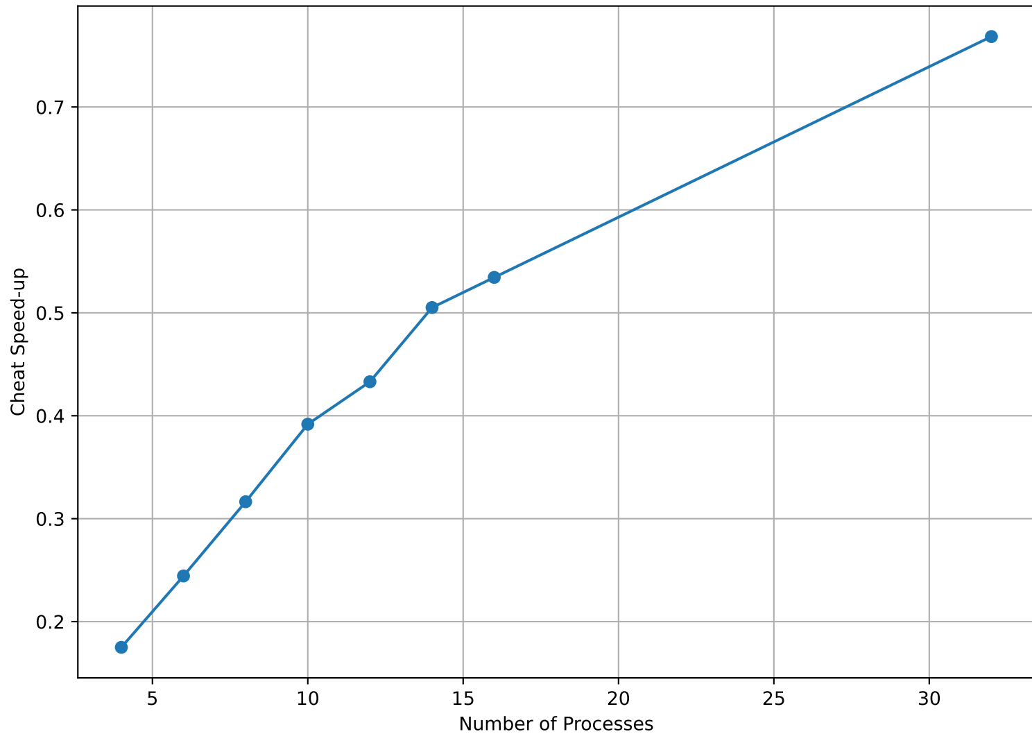
Cheat Wallclock Speed-up (3D harder)
